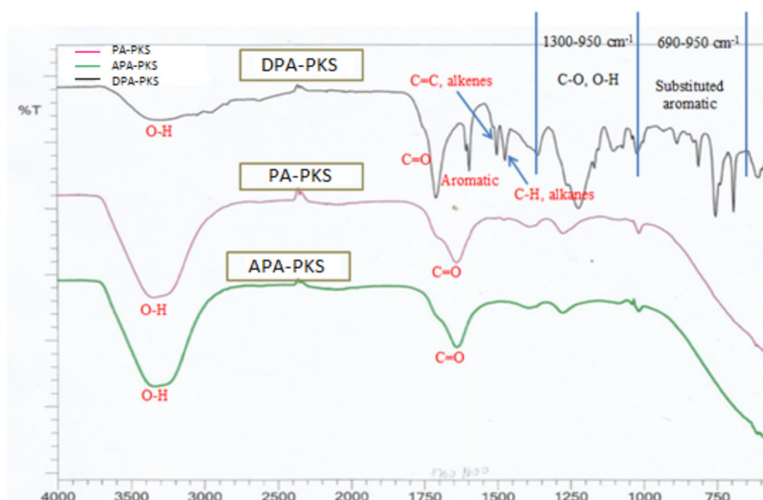
FIGURE 3. FTIR spectrum of DPA-PKS, PA-PKS and APA-PKS
